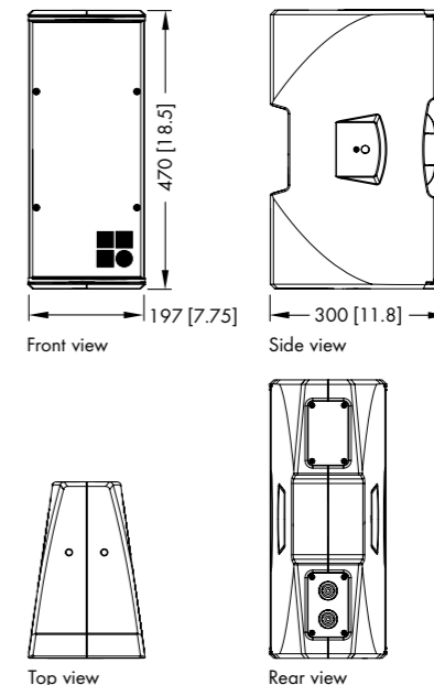
Ti10P cabinet dimensions in mm [inch]
